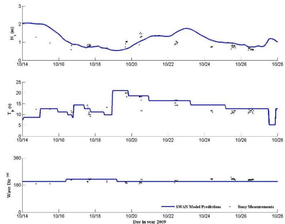
Figure 2. Model (line) representing the wave height ( H_s ), peak wave period ( T_p ) and mean wave direction (MWD) obtained from the Nearshore Santa Cruz SWAN model. Measured data (dots) were obtained from the Datawell DWR-G buoy deployed during the field study.
