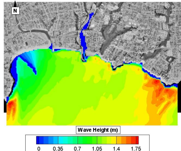
Figure 3. Peak wave heights in the model domain on 10/14/2009.
