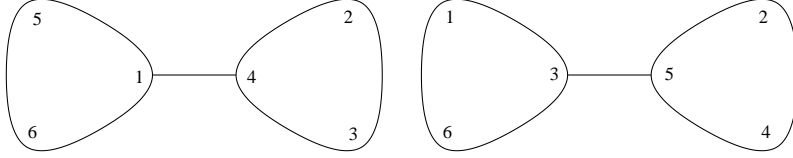
FIGURE 5. Two rank two labelled hypertrees in \text{HT}_6 .
