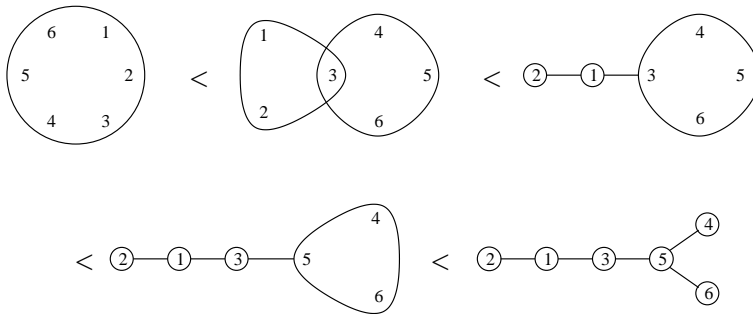
FIGURE 1. A maximal chain in \text{HT}_6 .
