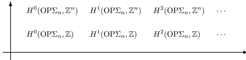
FIGURE 12. The E_2 page of the Lyndon-Hochschild-Serre spectral sequence for 1 \rightarrow \mathbb{F}_n \rightarrow P\Sigma_n \rightarrow OP\Sigma_n \rightarrow 1 .
