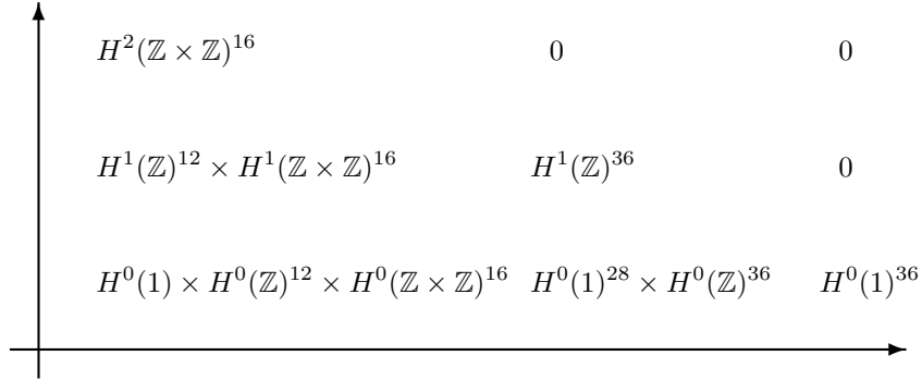
FIGURE 2. The E_1 page of the equivariant spectral sequence for the action OP\Sigma_4 \curvearrowright MM_n .
