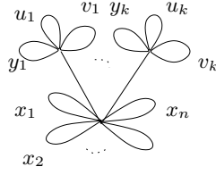
FIGURE 4. Graph giving the inclusion A_{n,k} \hookrightarrow \text{Aut}(F_{n+3k})
