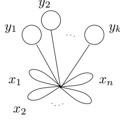
FIGURE 1. G_{n,k}
