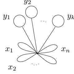
FIGURE 1. G_{n,k}
