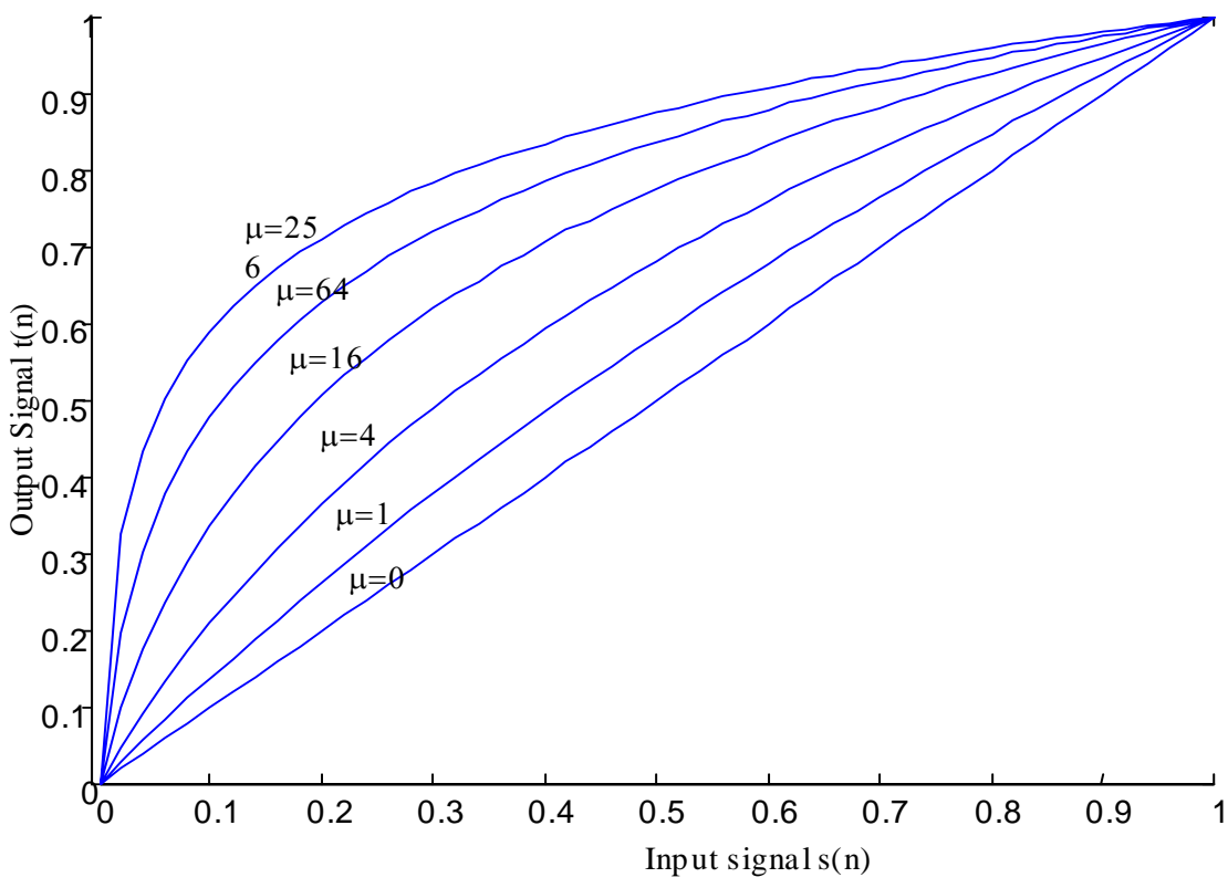
Figure 3.3 \mu -law companding function \mu=0, 4, 16 \dots 256 .
