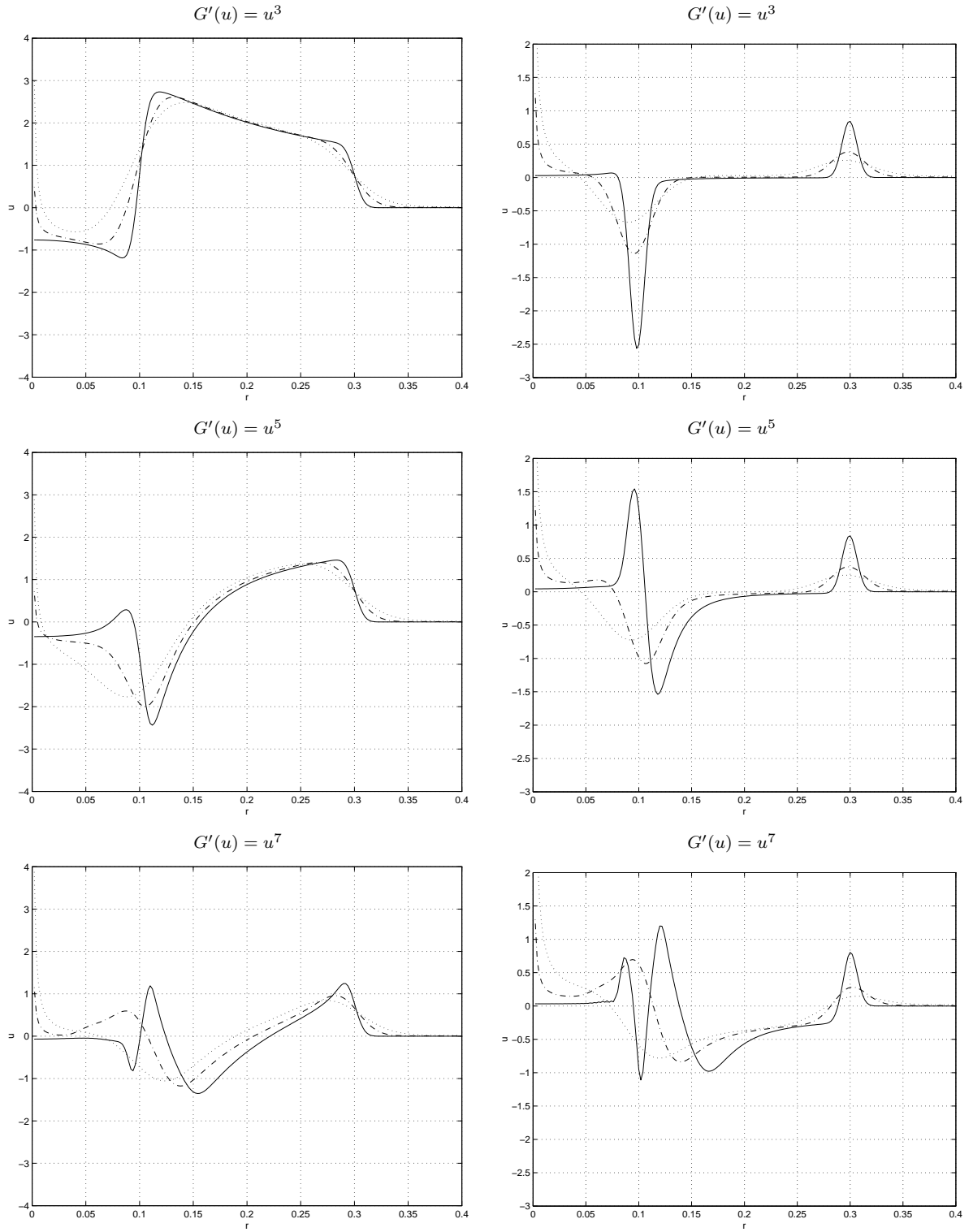
FIGURE 4.8: Approximate radial solutions for the Klein-Gordon equation with nonlinearity G'(u) at t = 0.2 for initial data \phi(r) = 0 , \psi(r) = 100h(r) (left column) and \phi(r) = h(r) , \psi(r) = 0 (right column), boundary condition u(0.4, t) = 0 , and \beta = 0 (solid), \beta = 0.001 (dashed), and \beta = 0.003 (dotted).
