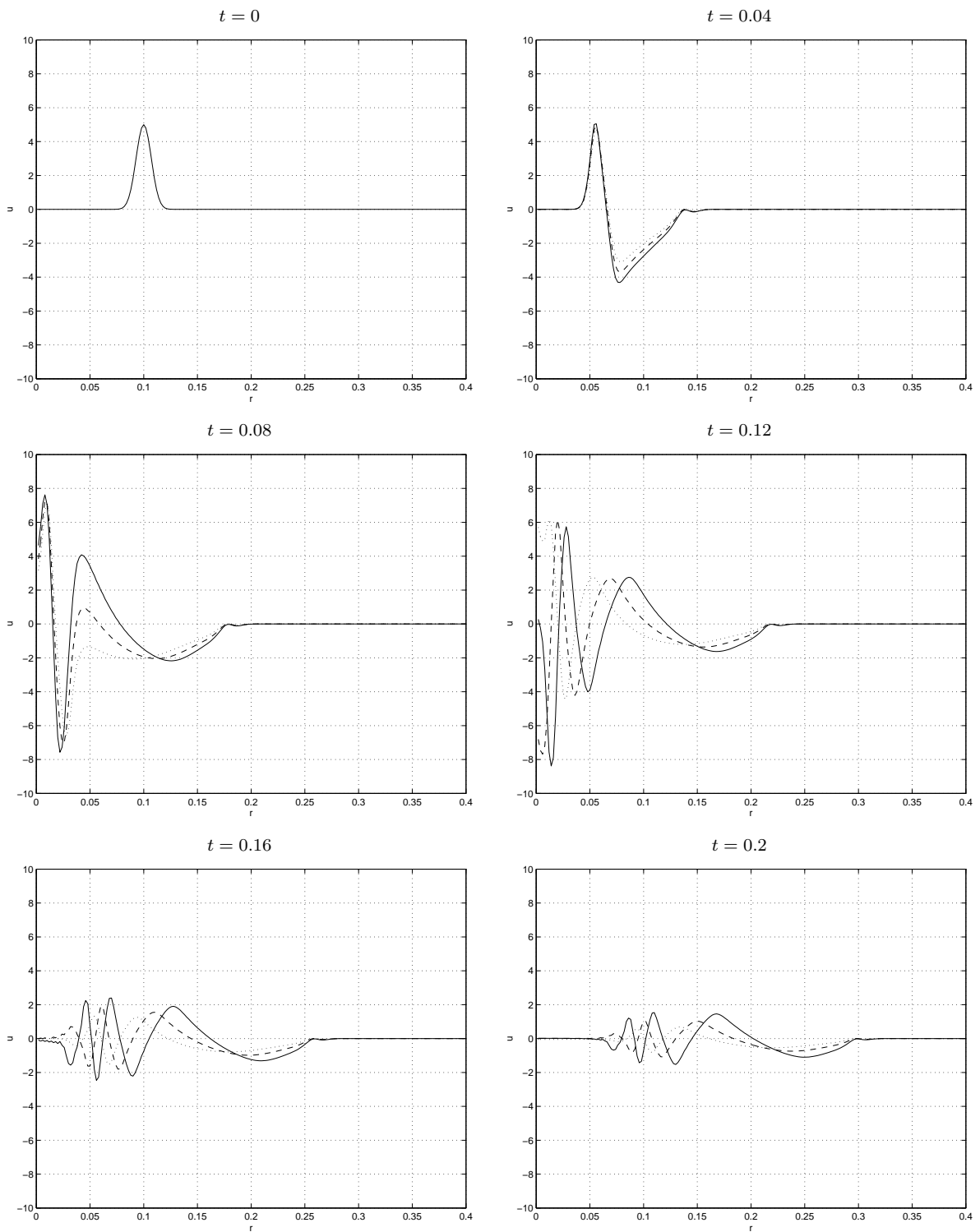
FIGURE 4.3: Approximate radial solutions at successive times of the undamped (solid line) and the damped nonlinear Klein-Gordon equation with \gamma = 5 (dashed line) and \gamma = 10 (dotted line), nonlinear term G'(u) = u^7 , initial data \phi(r) = h(r) , \psi(r) = h'(r) + h(r)/r , and boundary condition u(0.4, t) = 0 .
