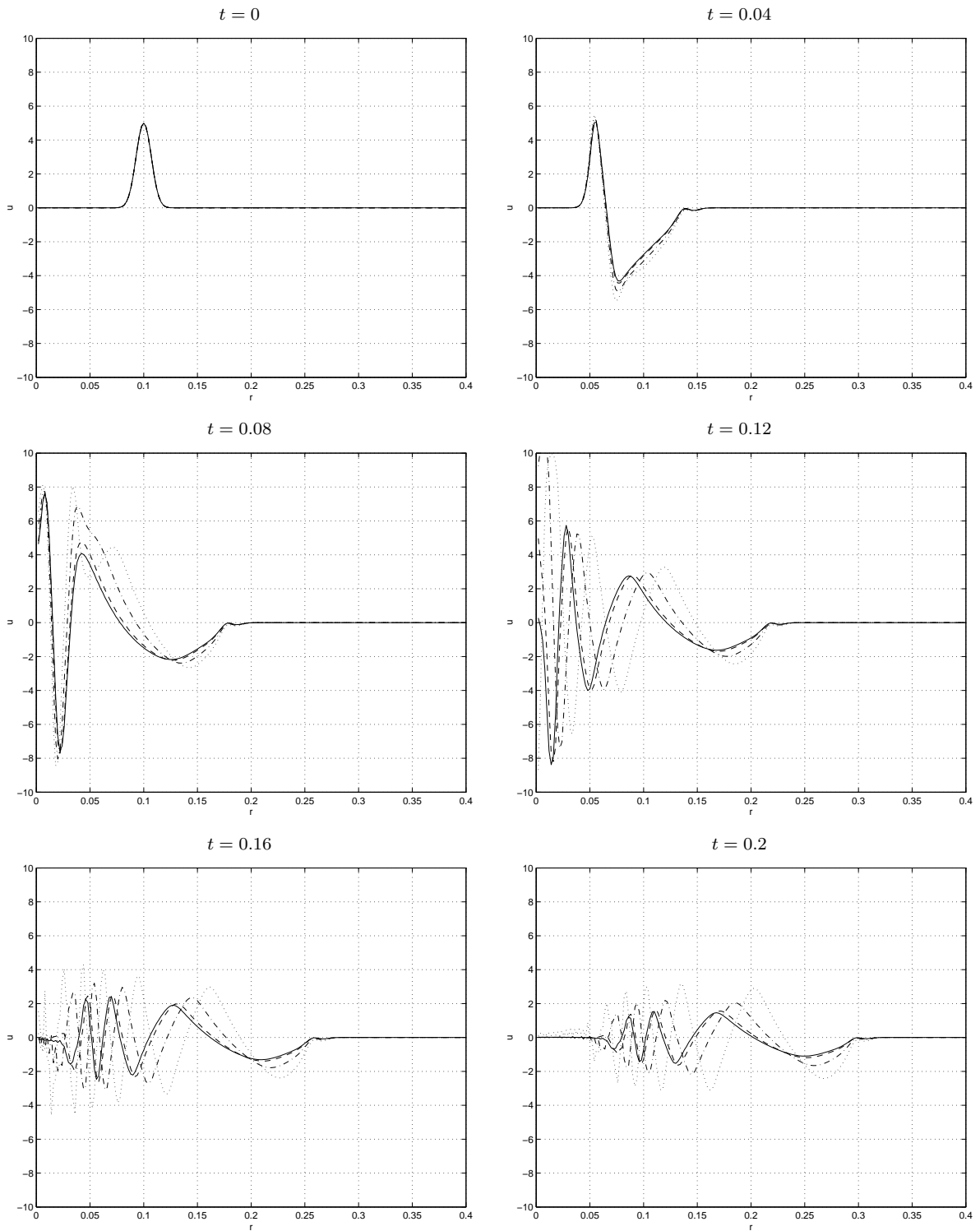
FIGURE 4.5: Approximate radial solutions at successive times of the undamped (solid) and the damped nonlinear Klein-Gordon equation with \gamma = -1 (dashed), \gamma = -5 (dash-dotted), and \gamma = -10 (dotted), nonlinear term G'(u) = u^7 , and initial data \phi(r) = h(r) , \psi(r) = h'(r) + h(r)/r , and boundary condition u(0.4, t) = 0 .
