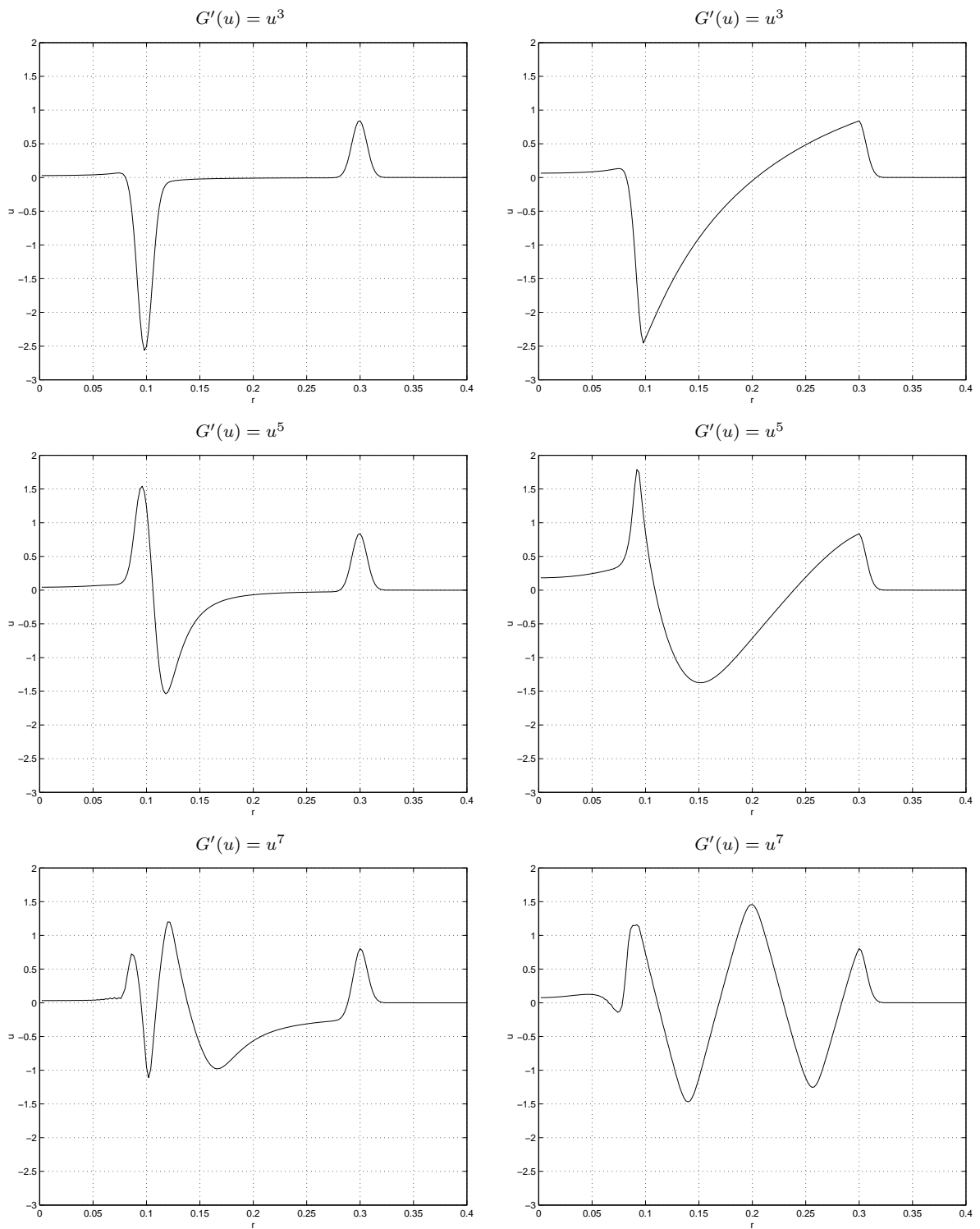
FIGURE 3.4: Approximate radial solutions for the given function G'(u) at time t = 0.2 for initial data \phi(r) = h(r) , \psi(r) = 0 on the left column, and initial conditions (3.8) on the right column.
