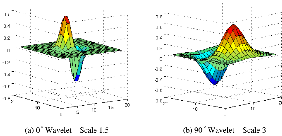
Figure 3.1: Wavelet illustration
